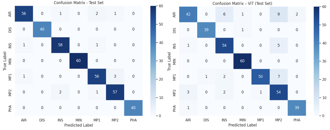
Fig. 2: Confusion Matrix - Results for VGG-16 and Transformer (Block = 50 ms)
