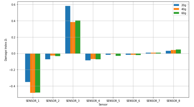
Fig. 4. Damage index per Sensor and Mass
