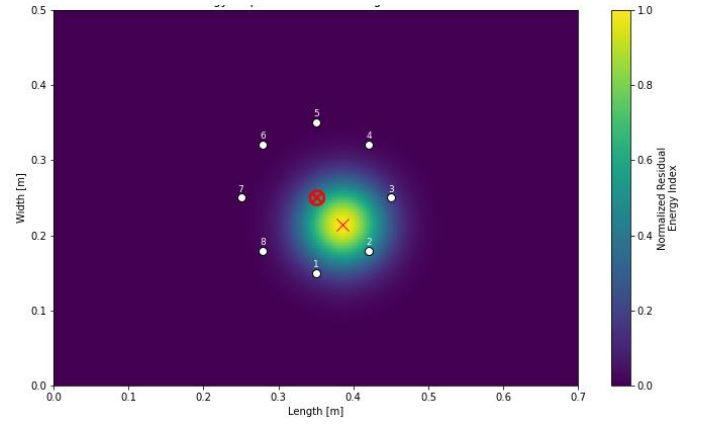
Fig. 6. Residual Energy Map
