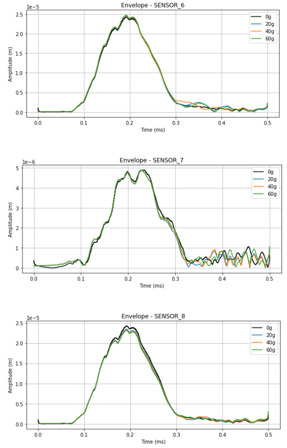
Fig. 3. Envelope Sensors
